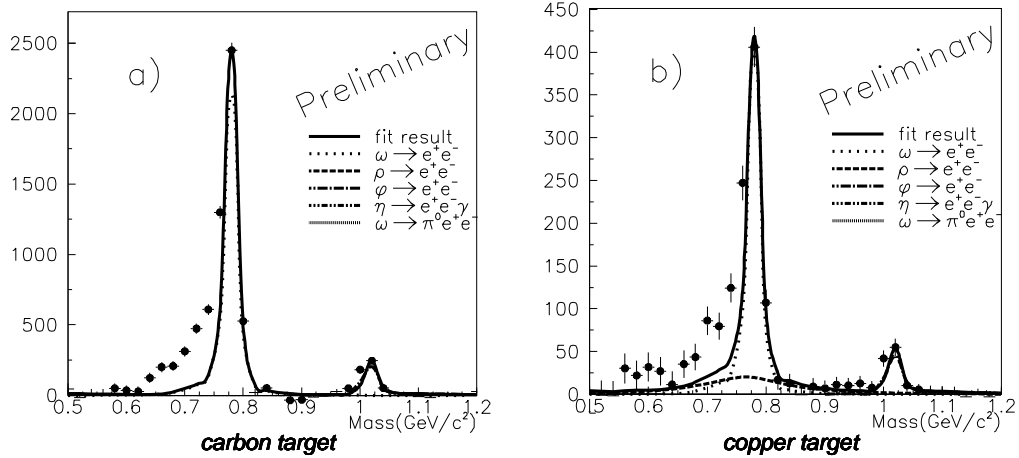
Figure 1: Invariant mass spectra of 2002 e^+e^- data, after the subtraction of the combinatorial background; a) is for the carbon target and b) is for the copper targets.
